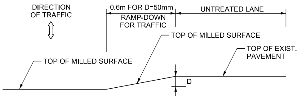
TEMPORARY LONGITUDINAL RAMP-DOWN/UP FOR MILLING OF ASPHALT PAVEMENT
