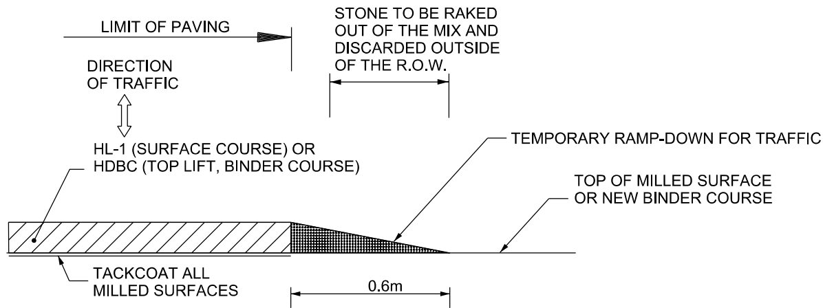
TEMPORARY LONGITUDINAL RAMP-DOWN OF BINDER COURSE OR SURFACE COURSE PAVING
